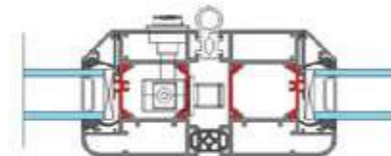
Interlock Detail
