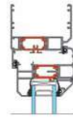
Head Detail
